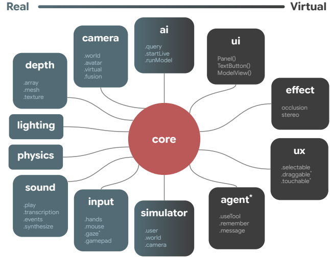
Figure 4: The modular architecture of the XR BLOCKS’s Script engine. The core engine consists of essential subsystems to realize the framework’s high-level abstractions, spanning perception (depth, input), AI integration (ai, agent), and user experience (ui, ux). Subsystems with * have not yet been fully implemented in the GitHub. While we show a few examples in XR Blocks, many implementations are far from perfection.
